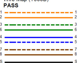
Wire Map (T568B)
