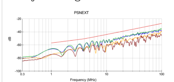
Limit Margin : 5.900 dB @ 1.001 MHz
